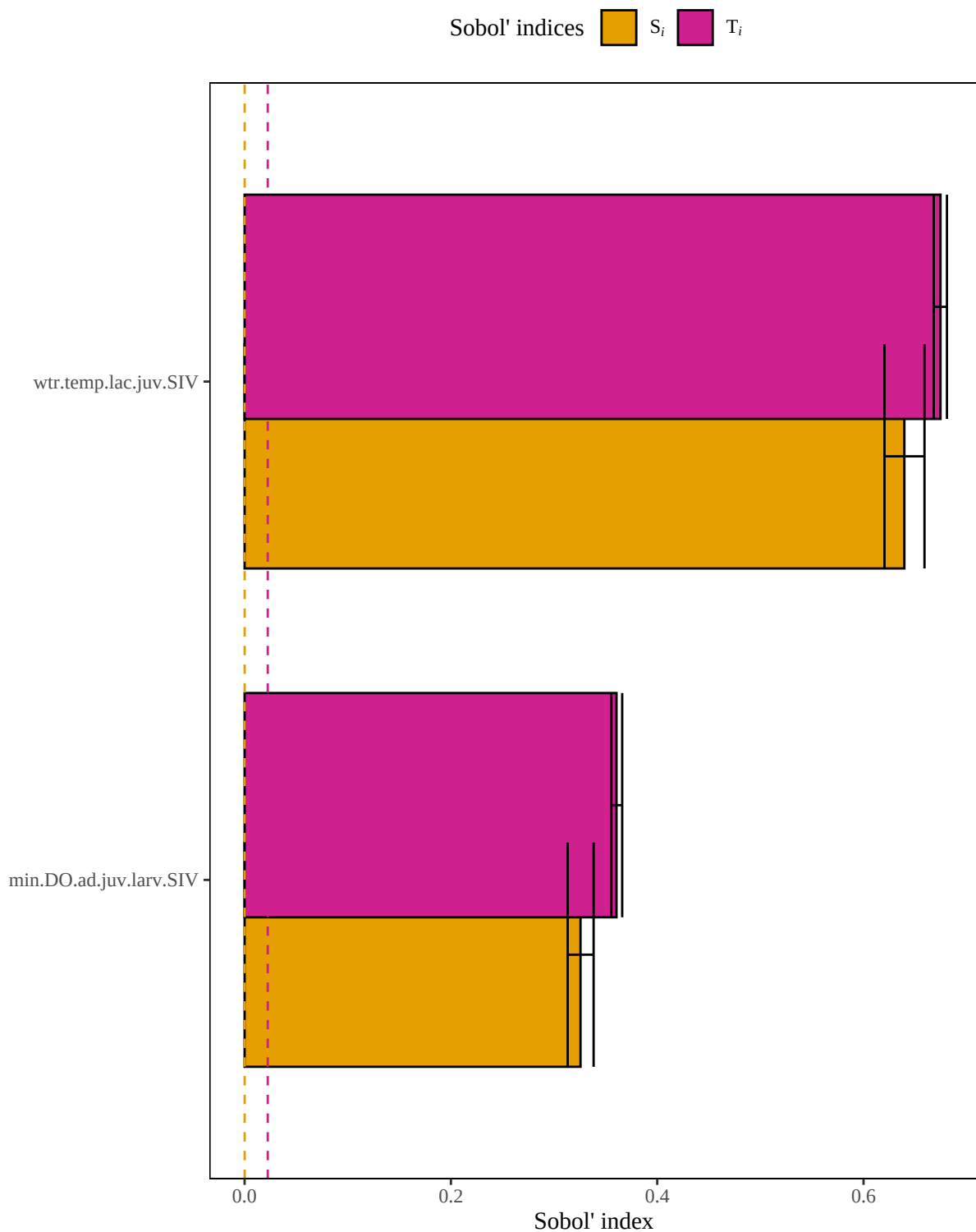
Figure 5. Results of a sensitivity analysis for the striped bass Inland Lac Juv model based on a geometric mean structure. Dashed lines represent baseline numerical approximation error for S_i and T_i ( i.e. , dummy variables).
